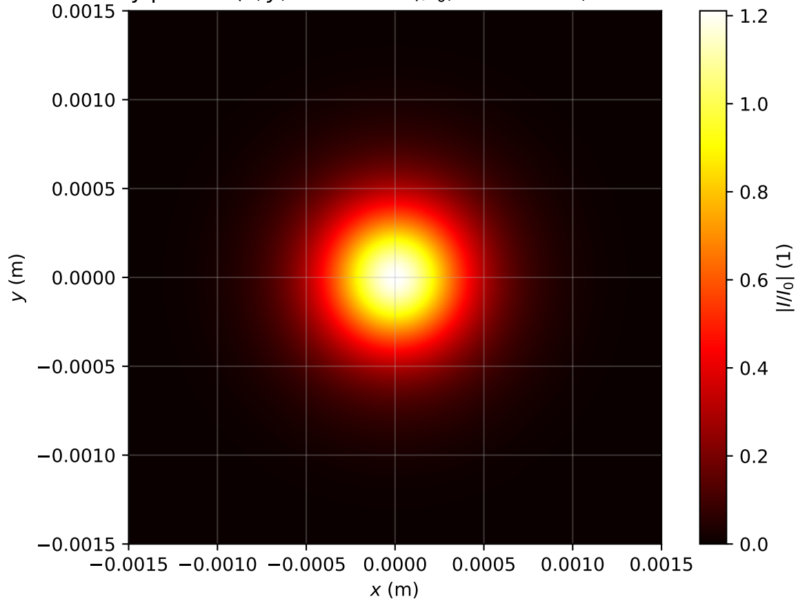
Intensity profile I(x, y, z = 1.274m)/I_0 , Pin=0.7Pcr, artificial time
